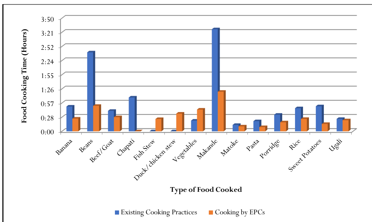
Chart 14: Time Taken to Cook by Food Types (Existing and EPC Practices)
