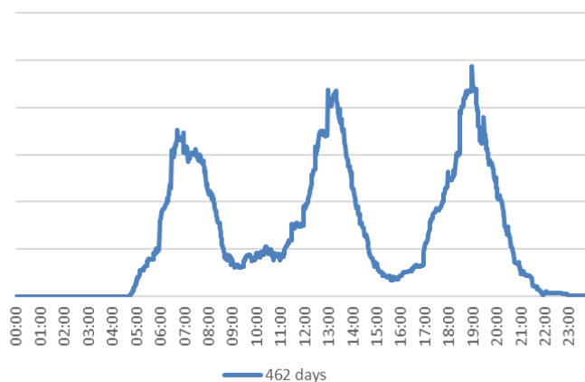
Figure 7: Average load profile for all complete days of data recorded during this study.
